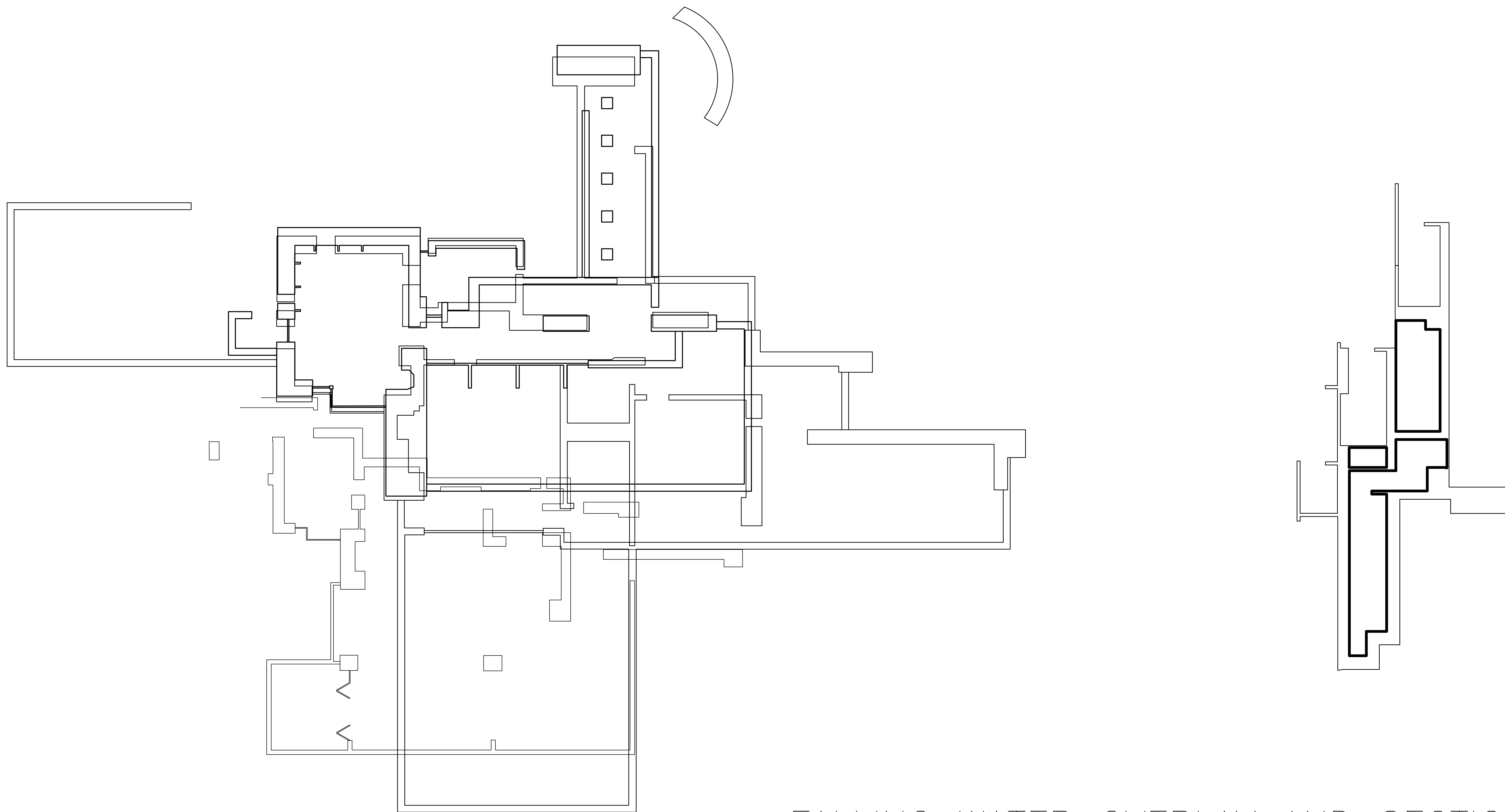
FALLING WATER OVERLAY AND SECTION ARCH1230_CLAYYOUUMAN_CHARLESIMNER ASSIGNMENT 15:SECTION DRAWING AND ANALYSIS SCALE: 1/8"=1'
