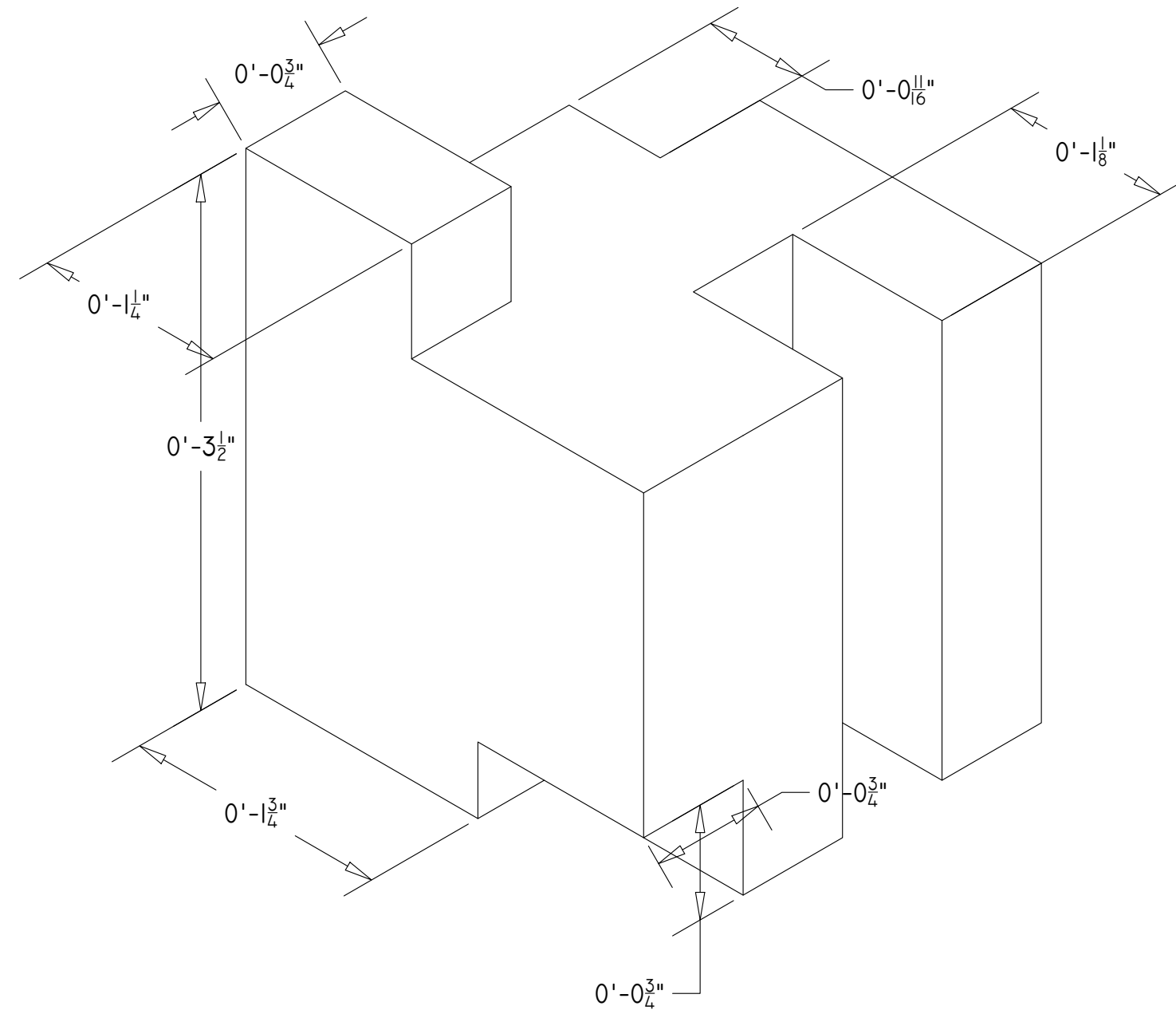
1 1 FRONT ISOMETRIC VIEW 1:1
