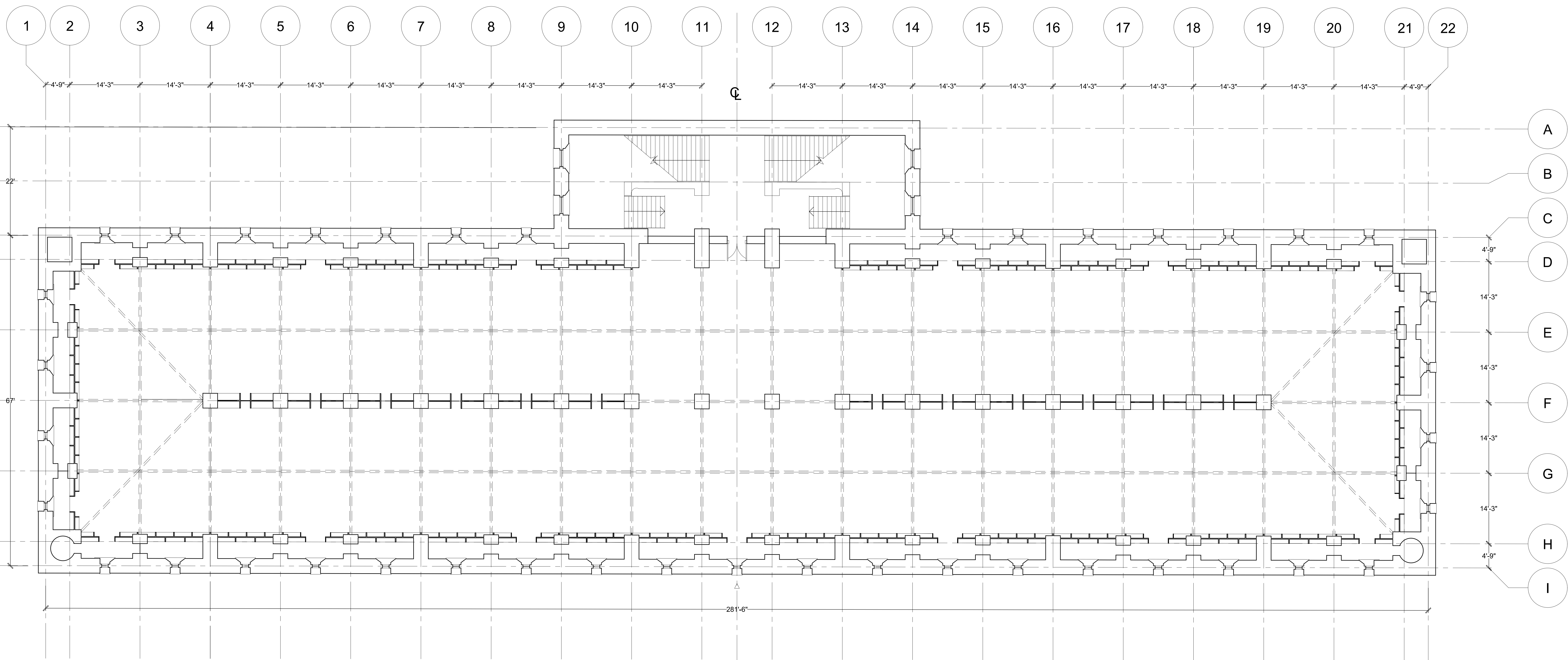
BIBLIOTHEQUE S. GENEVIEVE SECOND FLOOR PLAN ARCH 1230_MONTGOMERY_10-26-2017_VERA_BRYANT
