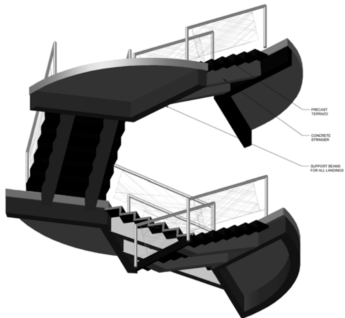
1 WORM'S EYE VIEW D-102/00 SCALE = 3/4" = 1'-0"
