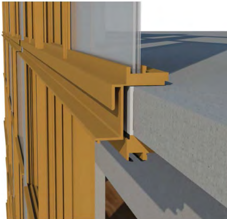
DETAIL AT FLOOR SLAB
