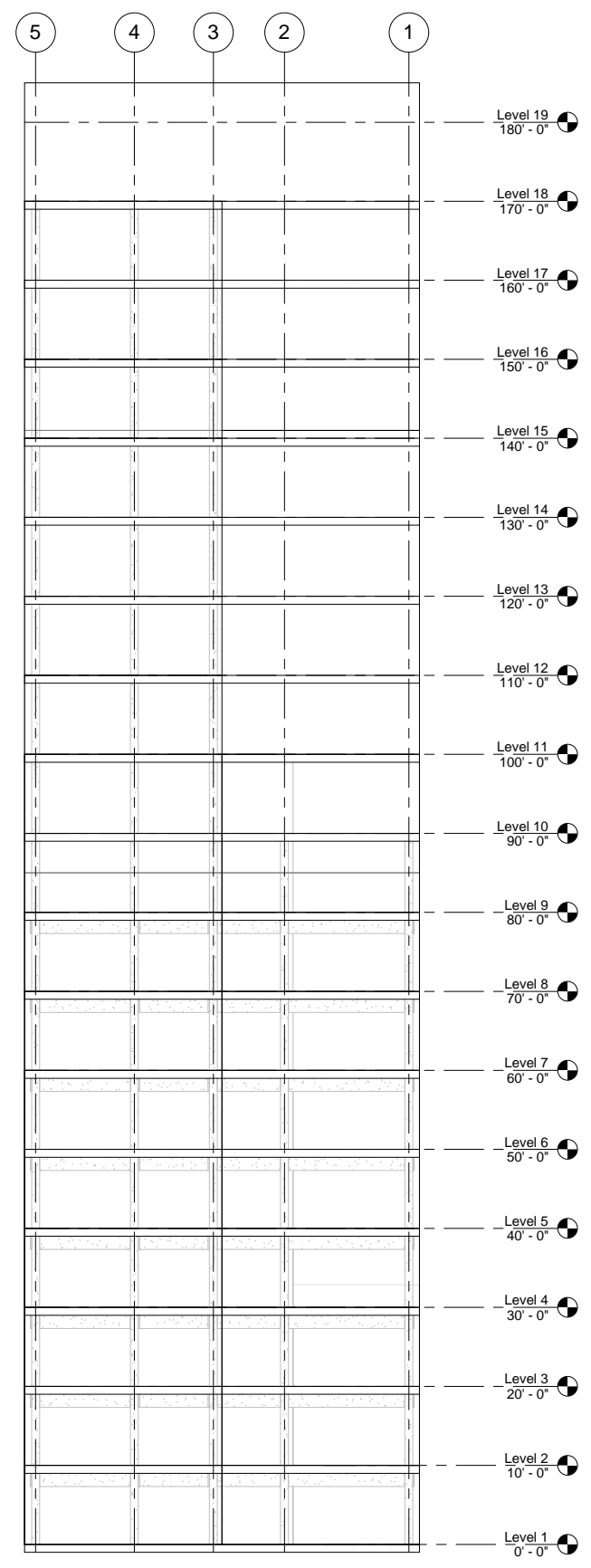
① North 1" = 10'-0"
