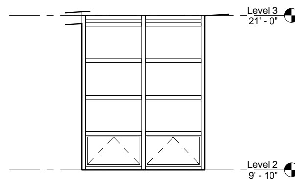
④ Window Section 1/4" = 1'-0"
