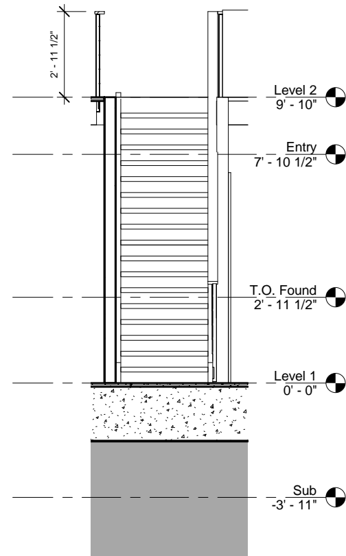
② stair section 2 3/8" = 1'-0"
