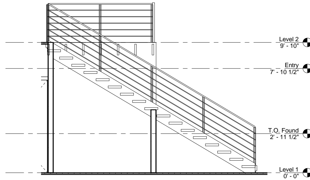
① Stair section 3/8" = 1'-0"
