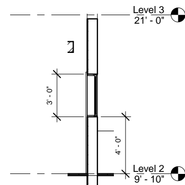
⑦ Window Section 3 1/4" = 1'-0"
