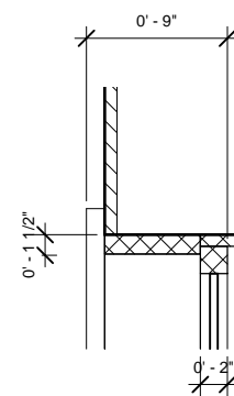
⑥ Window Section Detail 1 1/2" = 1'-0"
