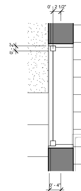
③ Window Plan 3 1" = 1'-0"
