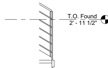
⑤ Railing 2 1/2" = 1'-0"
