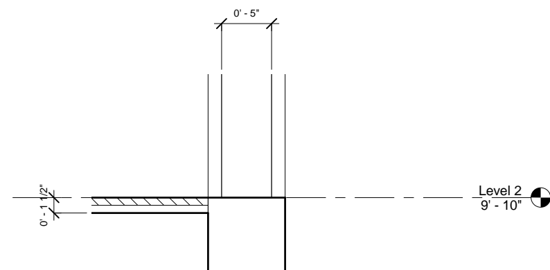
⑧ Window Section Detail 2 1 1/2" = 1'-0"
