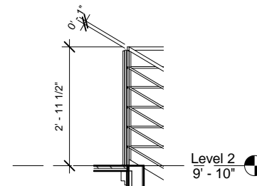
④ Railing 1/2" = 1'-0"
