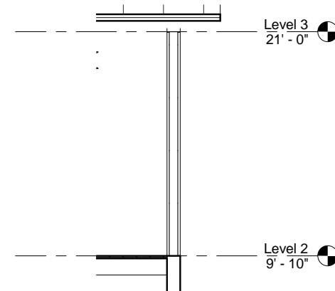
⑤ Window Section 2 1/4" = 1'-0"
