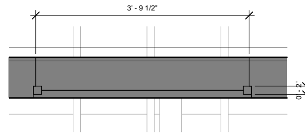
① Window Plan 2 1" = 1'-0"
