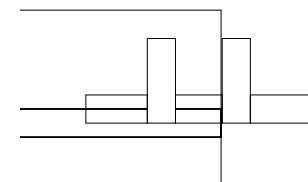
⑥ Railing Detail 6" = 1'-0"
