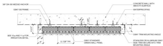
Green Wall Systems - Plan
