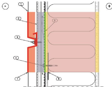
Rain Screen – Vertical Section
