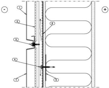
Manufacturer: Ruukki Elevations and Wall Sections
