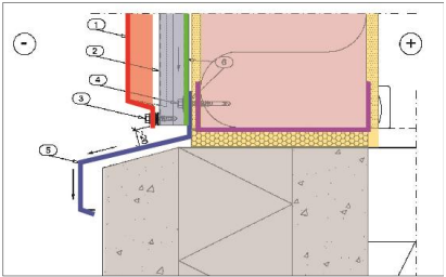
Rain Screen – Vertical Section
