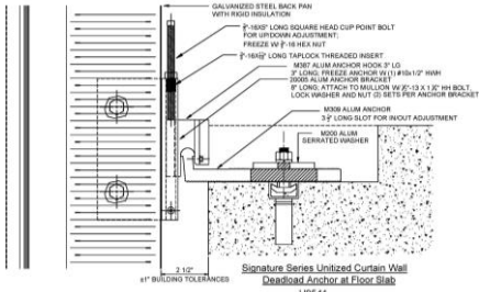
Glass - Unitized System Section
