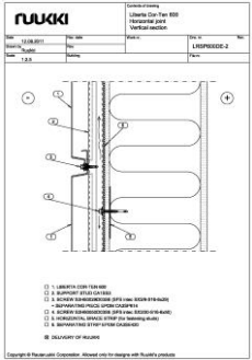
Manufacturer: Ruukki Elevations and Wall Sections
