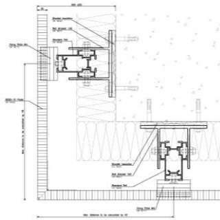
Manufacturer: Hunter Douglas Elevations and Wall Sections
