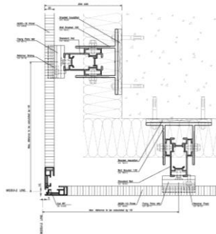
Manufacturer: Hunter Douglas Elevations and Wall Sections
