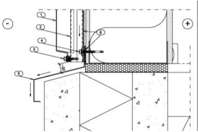
Rain Screen – Vertical Section
