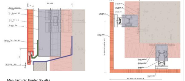
Manufacturer: Hunter Douglas Elevations and Wall Sections
