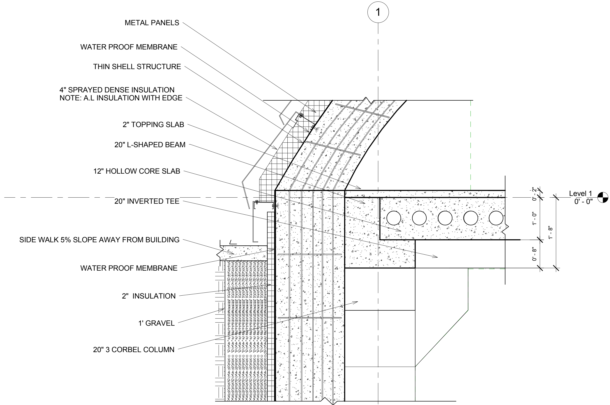
① TYP. DETAIL OF THIN SHELL AND FOUNDATION 1" = 1'-0"
