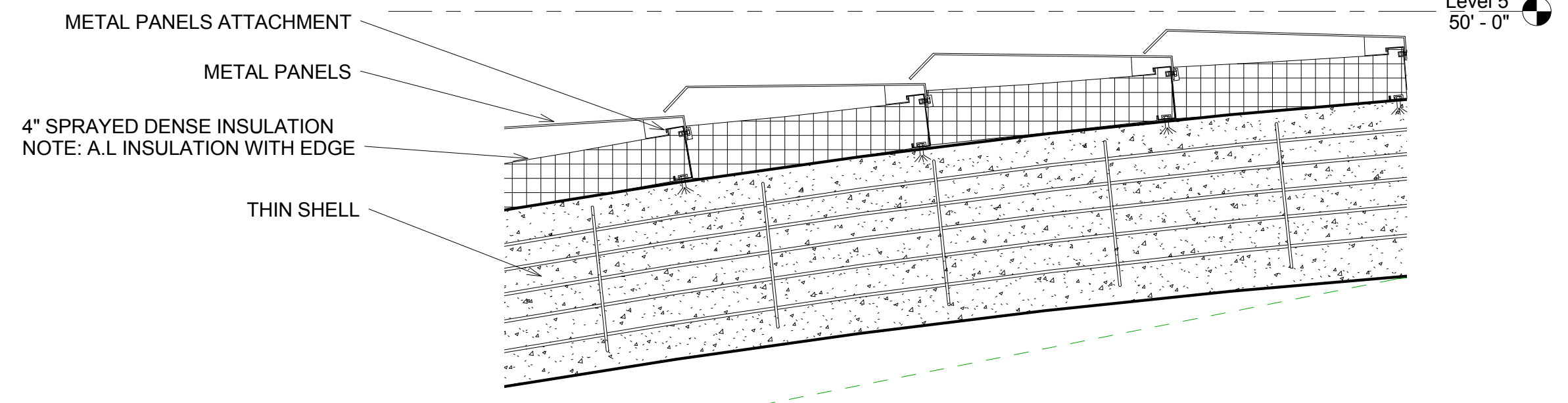
③ TYP. ASSEMBLY OF THIN SHELL MID-WAY 1" = 1'-0"
