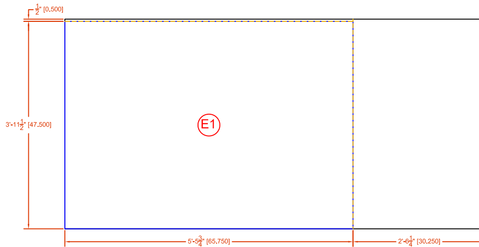
1/2" PLYWOOD BOARD
