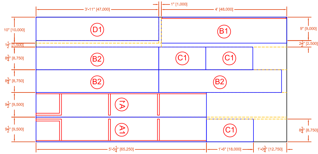
3/4" PLYWOOD BOARD
