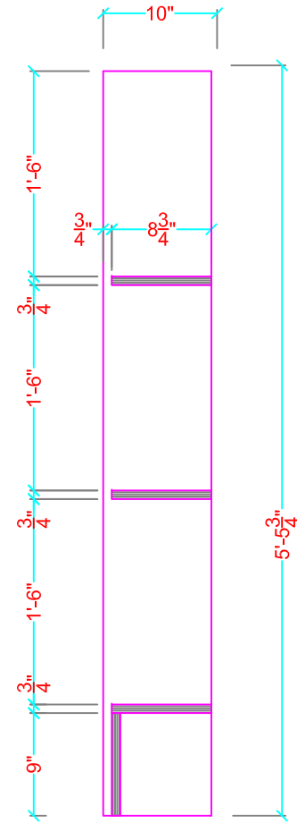
SECTION B-B
