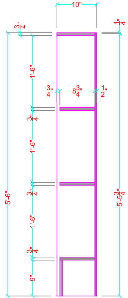
FRONT ELEVATION
