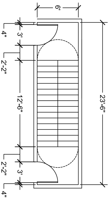
10' floor to floor height - scissor stairs (need 1)
