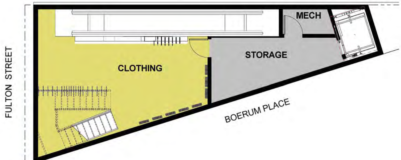
FLOOR PLAN-1ST FLOOR_CLOTHING
