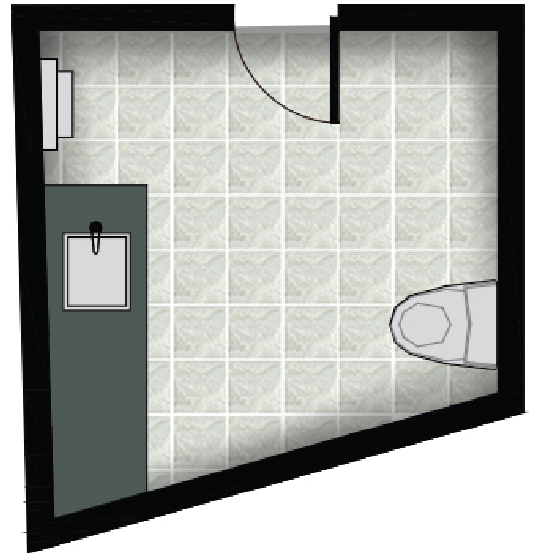
ADA BATHROOM FLOOR PLAN
