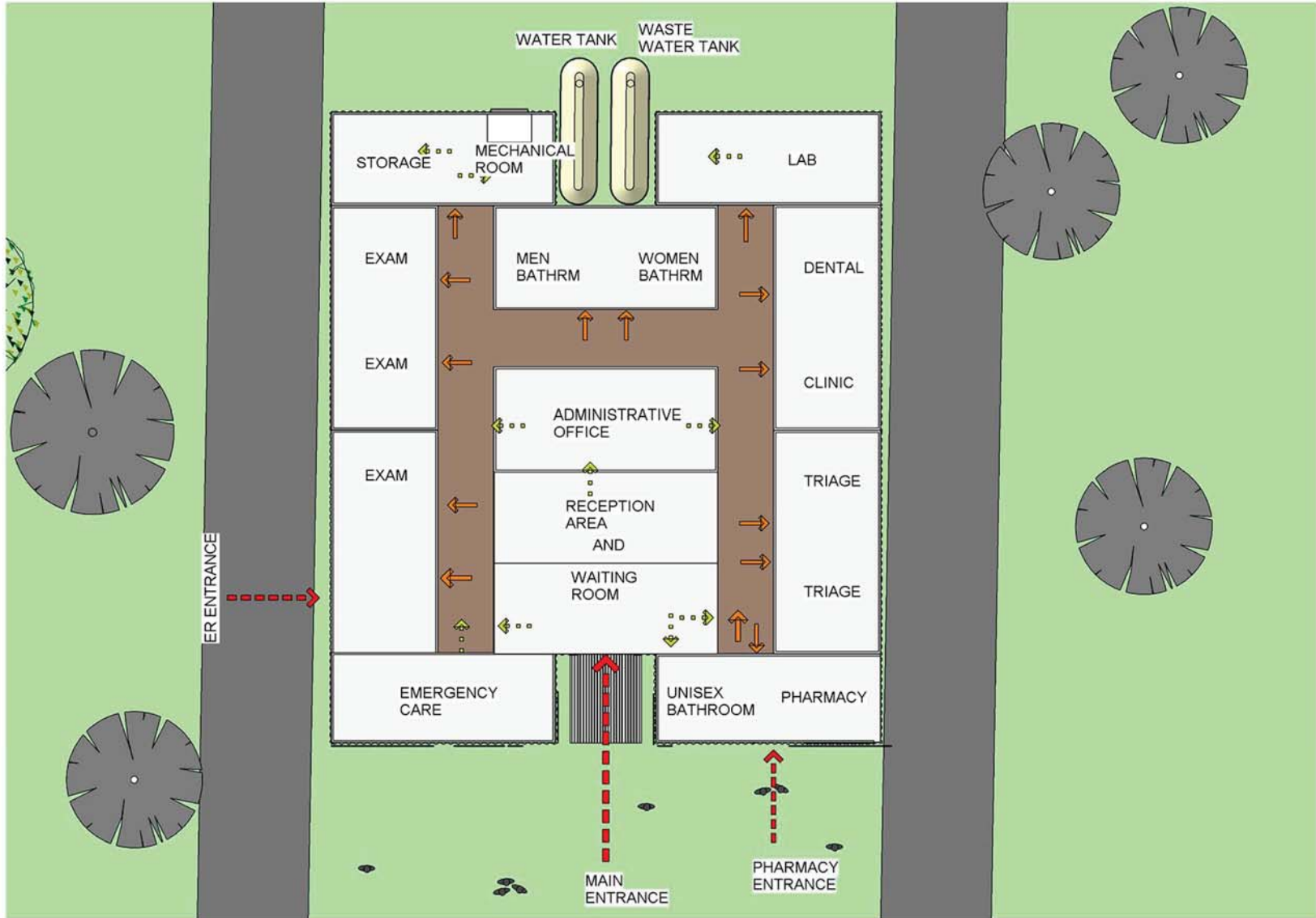
Site Plan
