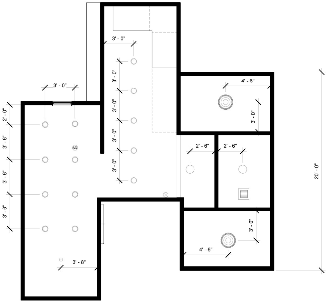
1 ST FLOOR RCP
