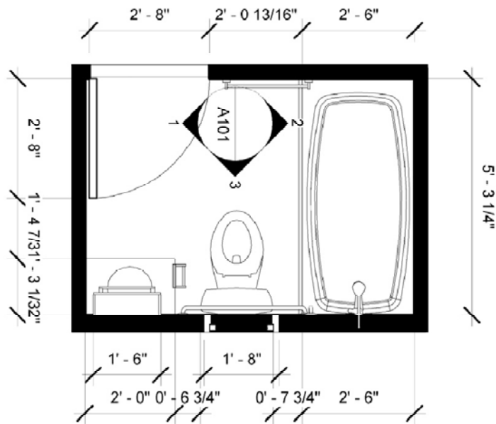
BATHROOM PLAN
