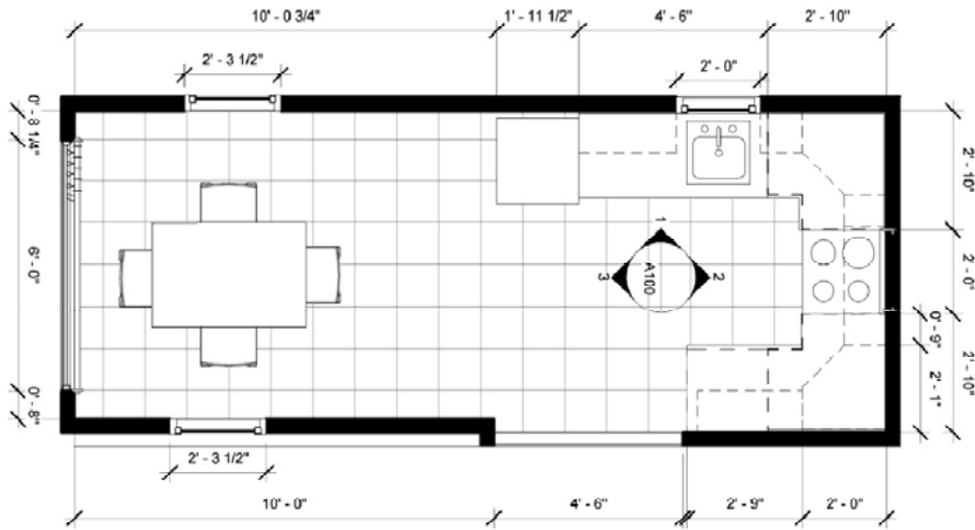
KITCHEN PLAN
