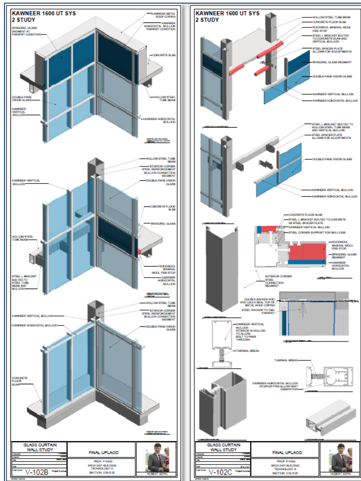
Sample Final Presentation – Vertical format – Glass Curtainwall (Courtesy of Hubert Szpin – Spring 2020)
