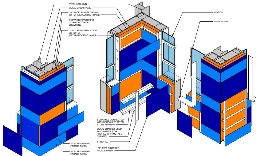
© ISO Outside Corner Installation
