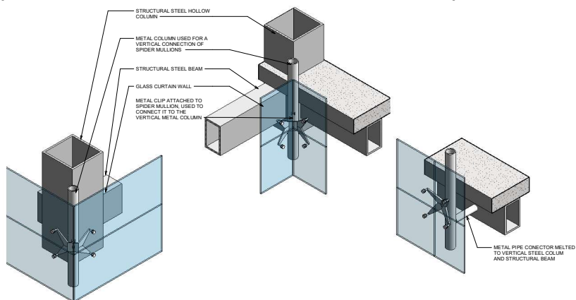
Wall Iso
