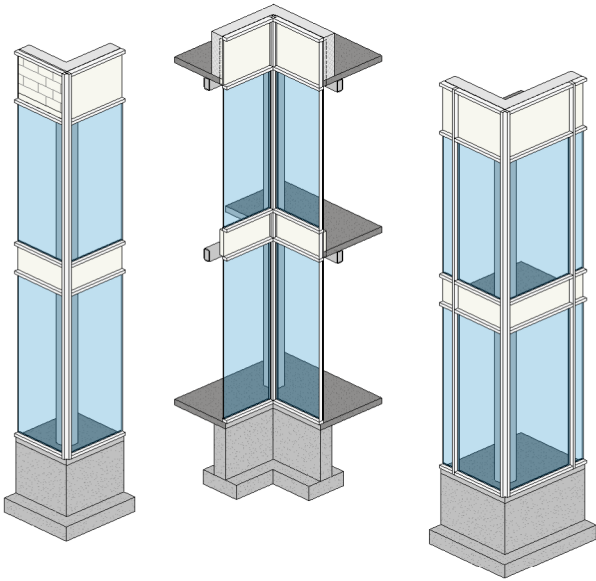
◎ CURTAIN WALL ANCHOR Glass 1 Glass 1
