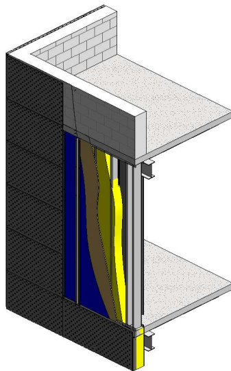
② Top Cladding Section
