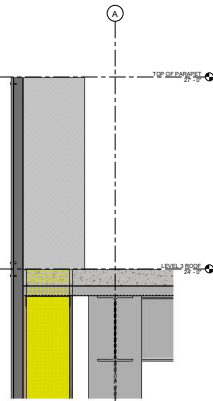
② Top Cladding Section
