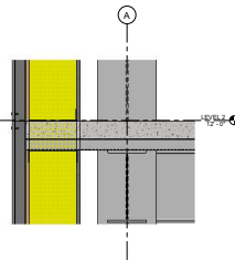
③ Main Cladding Section
