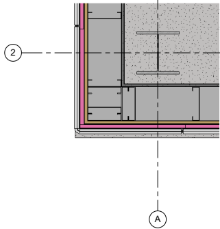
LEVEL 1 GROUND - Opaque - WALL PLAN SECTION 1 1/2" = 1'-0"
