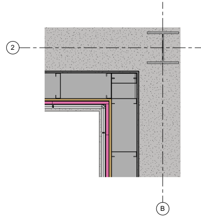
LEVEL 1 GROUND - Opaque - INNER CORNER WALL 1 1/2" = 1'-0"
