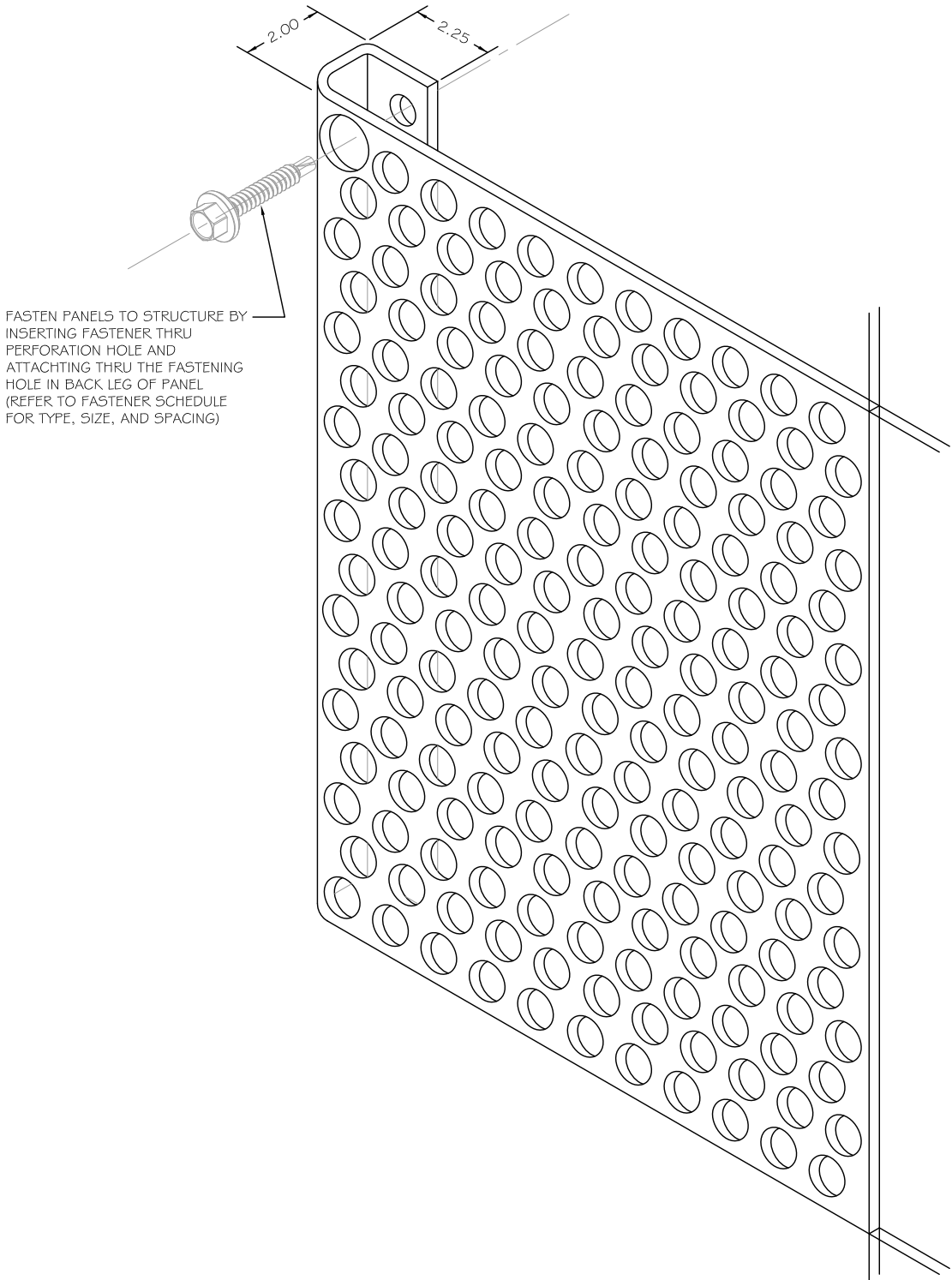
1 TYP PANEL FASTENING DETAIL
