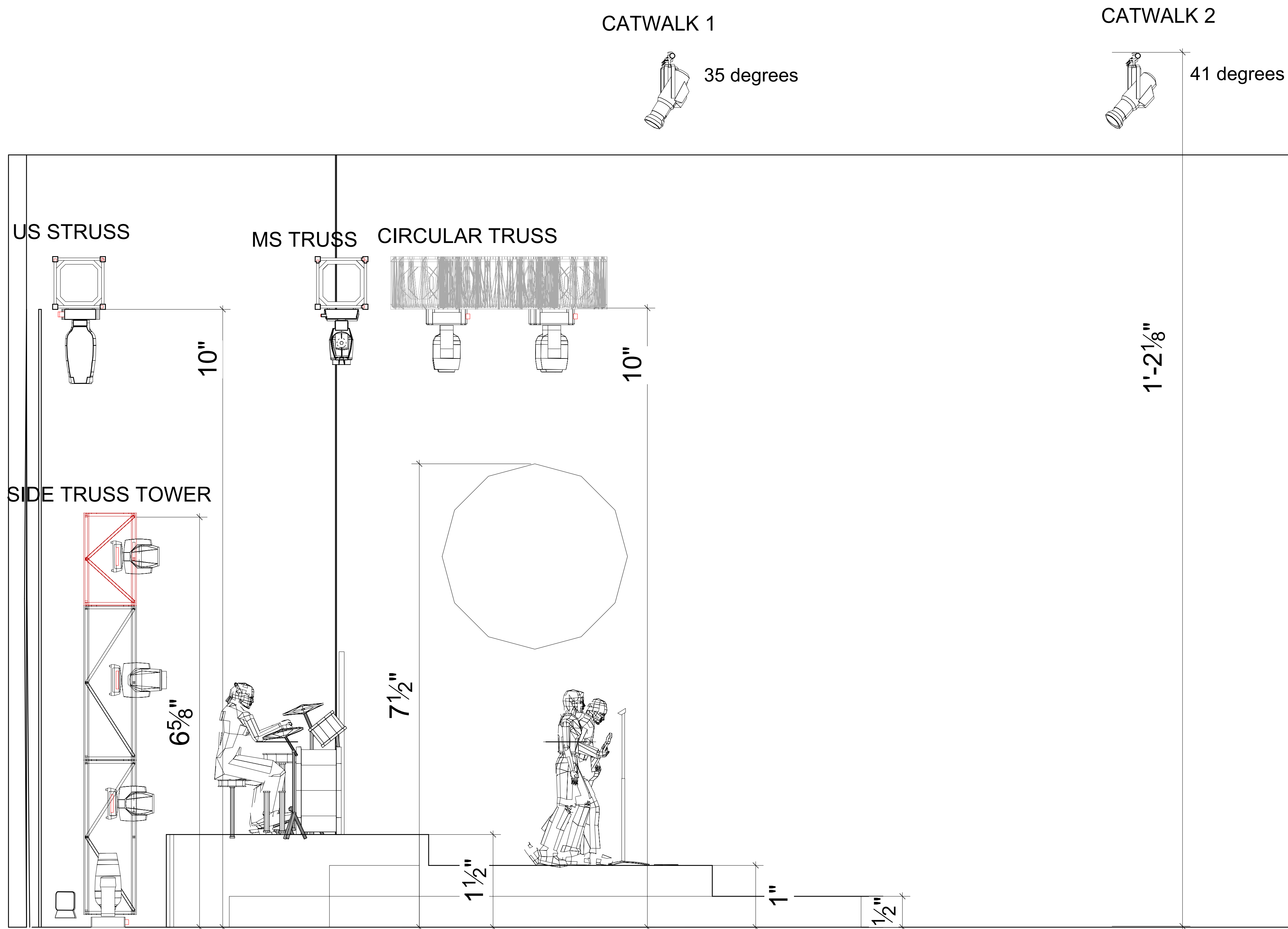
2 Section View Scale: 1/2" = 1'-0"
