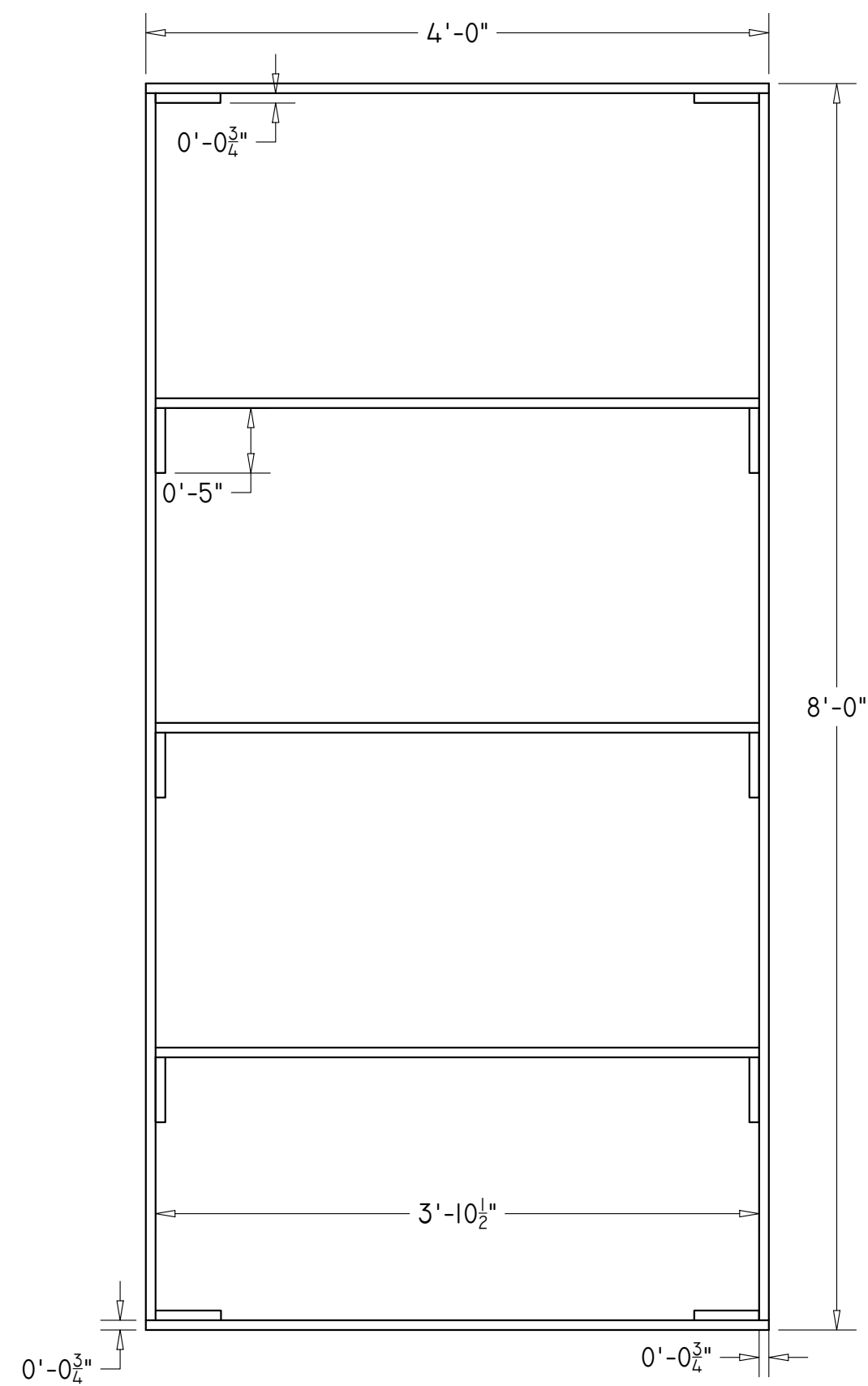
REAR
