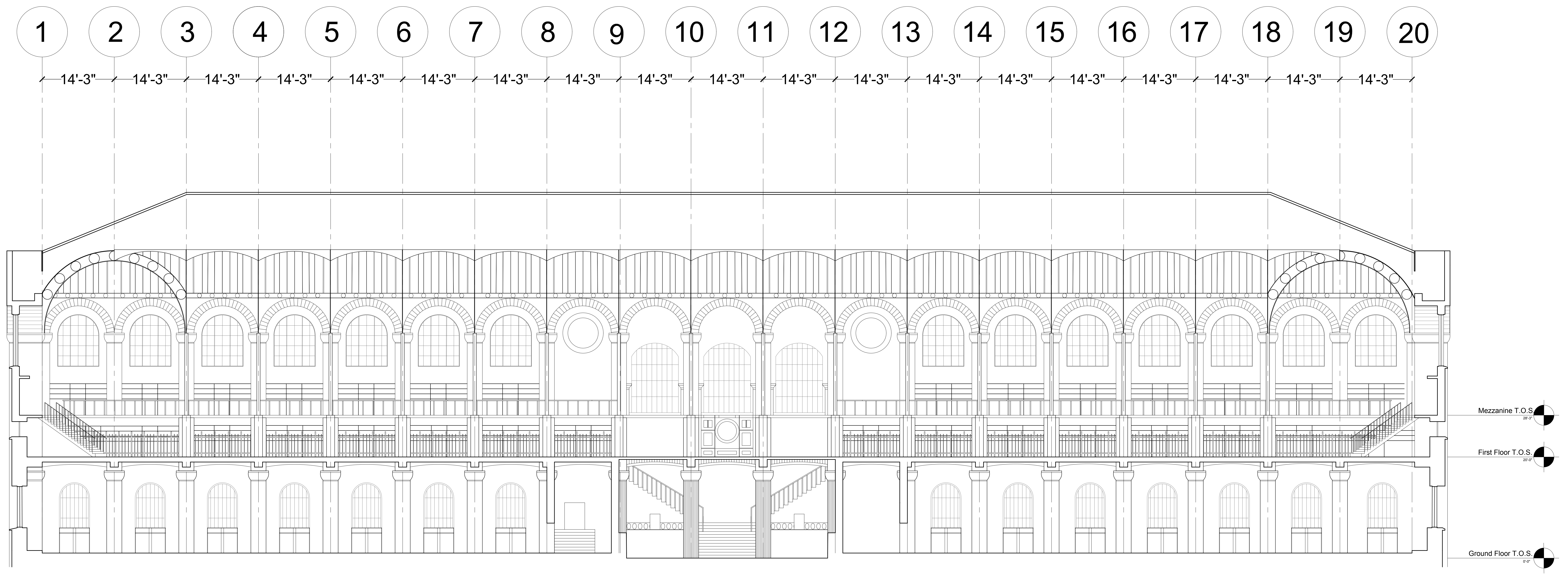
BIBLIOTHEQUE ST. GENEVIEVE LONG SECTION ARCH 1230 MONTGOMERY DECEMBER 14, 2017 ACEVEDO, ANTHONY
